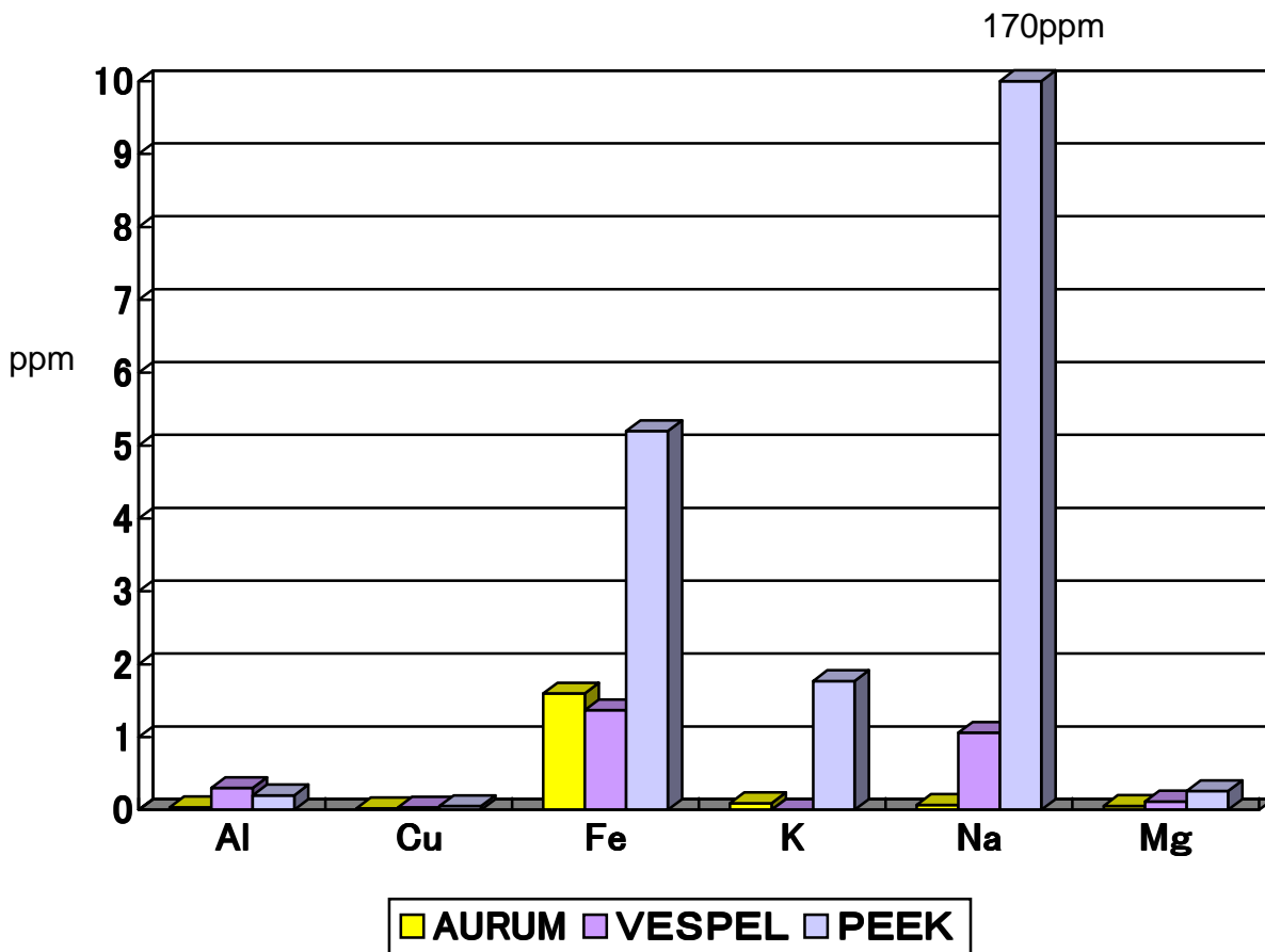
Fig. 1 Data on Analysis of Metallic Impurities
